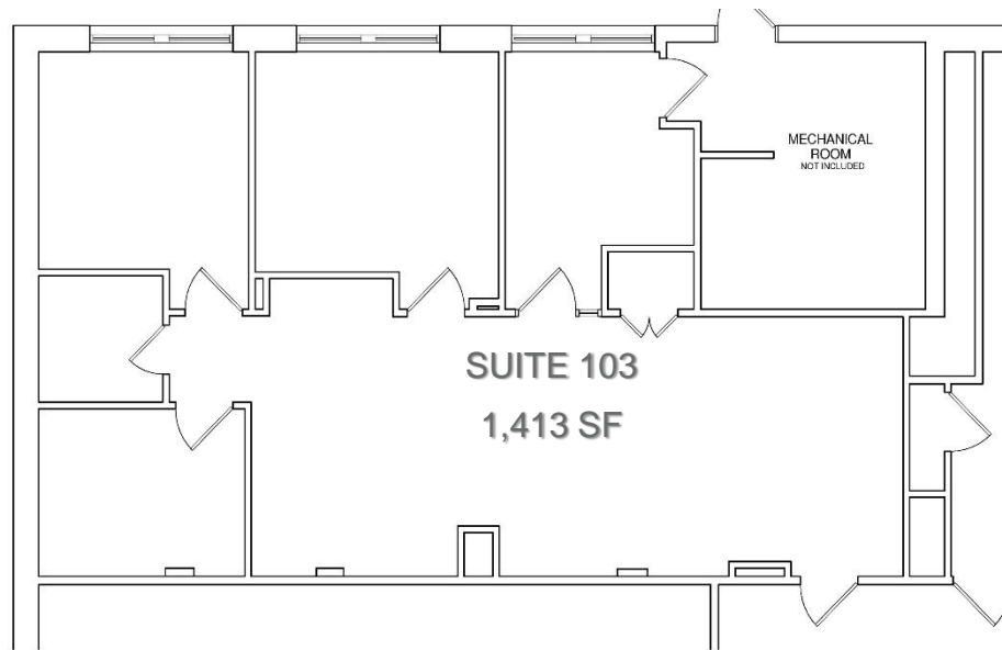
1 FIRST FLOOR EXISTING CONDITIONS PLAN 1/4" = 1'-0"
